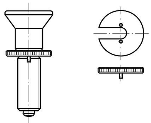
Indexing plunger with screw-in washer
